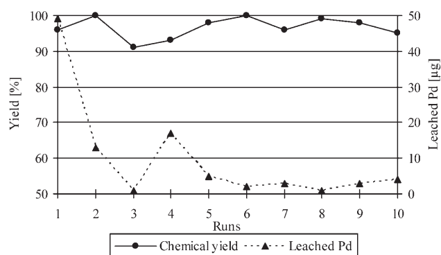
Figure 2. Chemical yield and amount of leached Pd using catalyst H .
