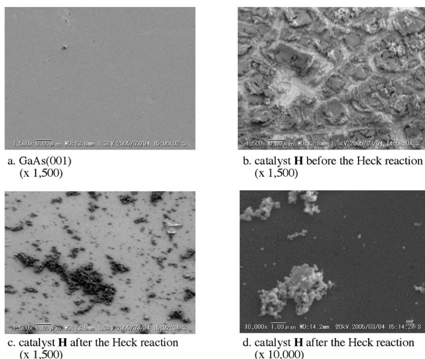
Figure 5. SEM observation of catalyst H .
