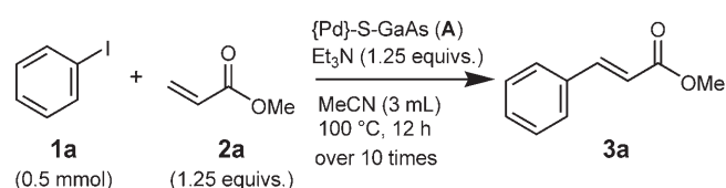
Scheme 1. Heck reaction.
