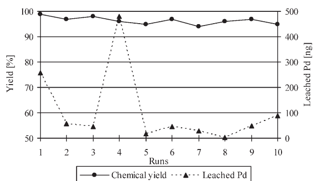
Figure 3. Chemical yield and amount of leached Pd using catalyst N . Unit of leached Pd is ng not \mu\text{g} .
