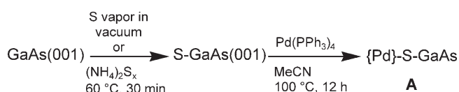
Figure 1. Preparation of three-phase catalyst, {Pd}-S-GaAs(001), catalyst A.
