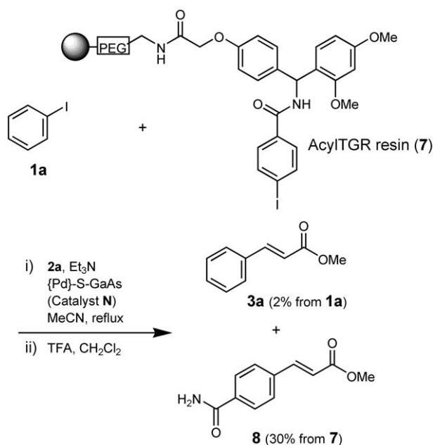
Scheme 2. Three-phase test.
